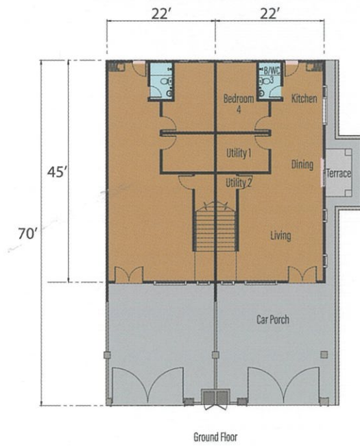
Type 22'x70' Floor Plan A
