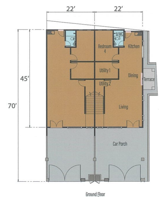
Type 22'x70' Floor Plan B
